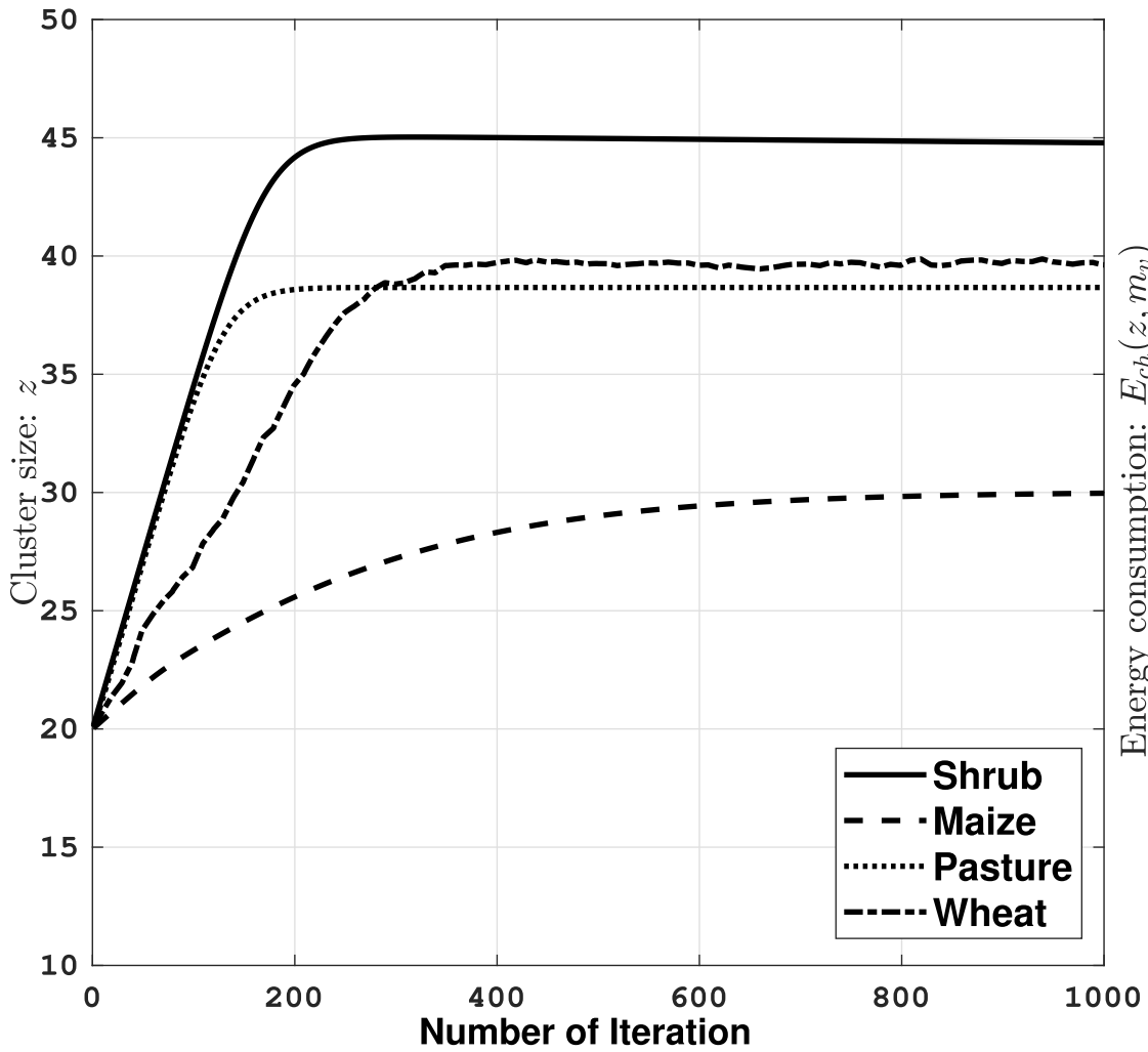
(a) Cluster Size vs. Iteration#
