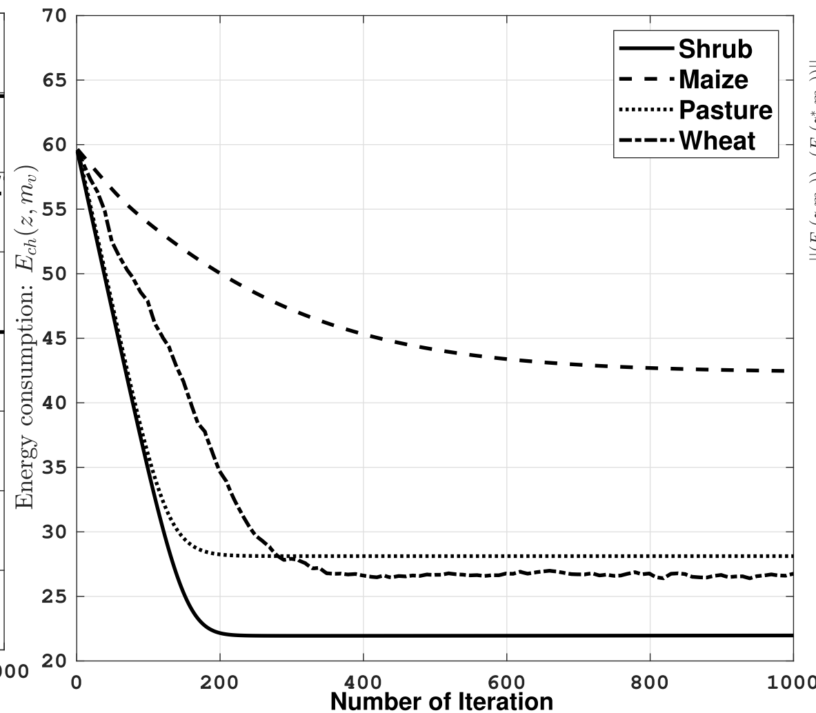
(b) Energy consumption vs. Iteration#
